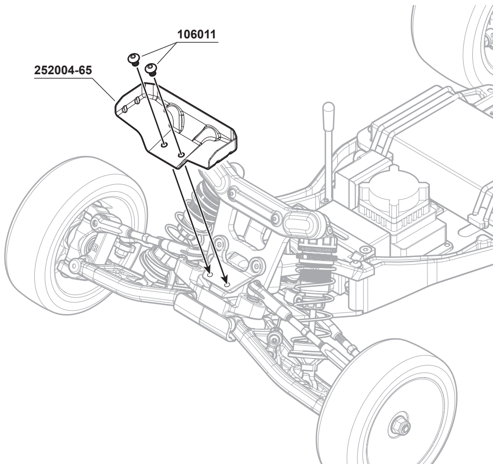
106011 M3x4mm Hex Scket OH/ST Screw x2
